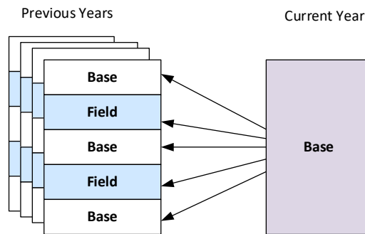
Figure 3.5. STAAR Common-Item Post-Equating Design
