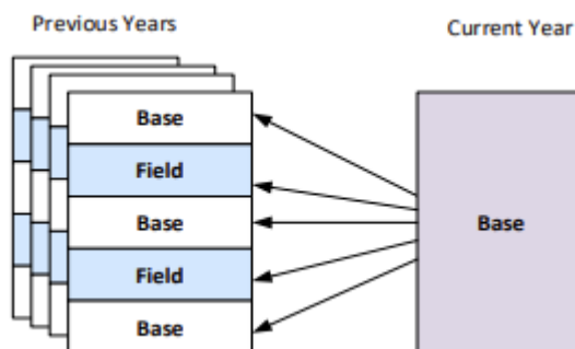
Figure 3.5. STAAR Common-Item Post-Equating Design
