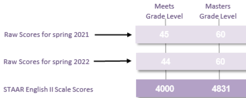
Figure 3.1. Relationship Between Raw Scores and Scale Scores at the Performance Standards
