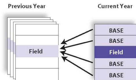
Figure 3.4. STAAR Alternate 2 and TELPAS Common-Item Post-Equating Design
